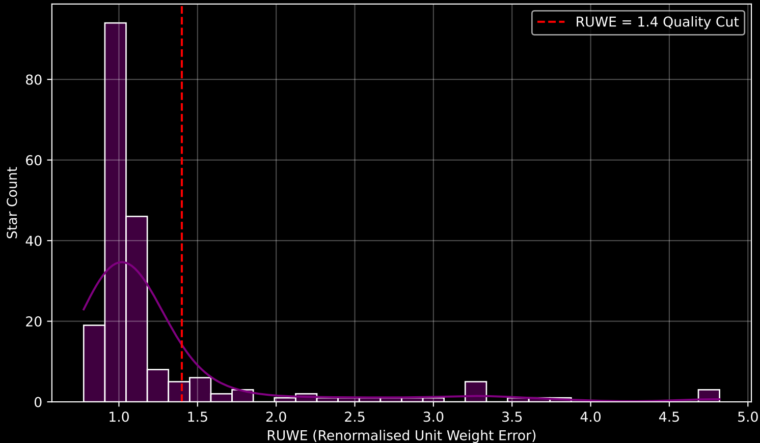
GAPOGEE DR17 Field [082+57_MGA] RUWE Distribution (n= 203)
