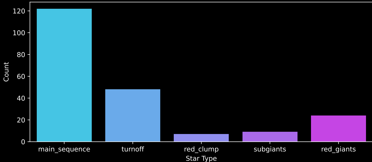
APOGEE DR17 Field: [082+57_MGA] Count plot of Star Type
