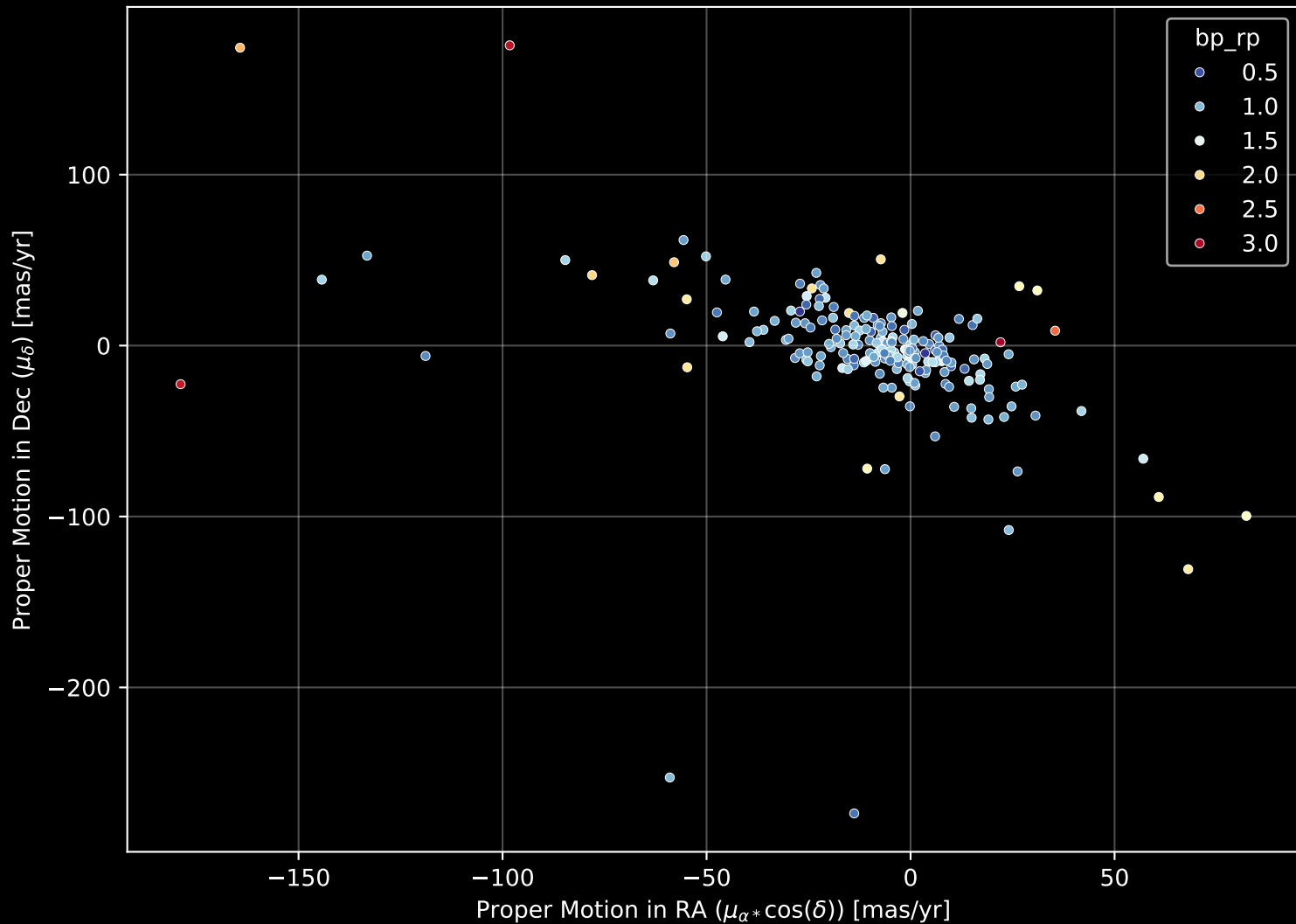
APOGEE DR17 Field: [082+57_MGA] Proper Motion Diagram (n= 210)
