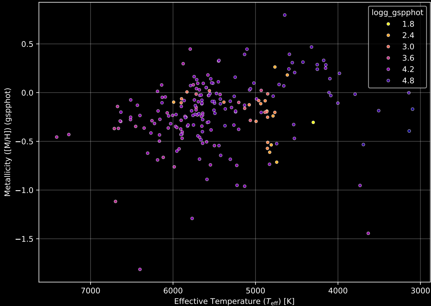
APOGEE DR17 Field: [082+57_MGA] Stellar Population Parameters (n= 210)
