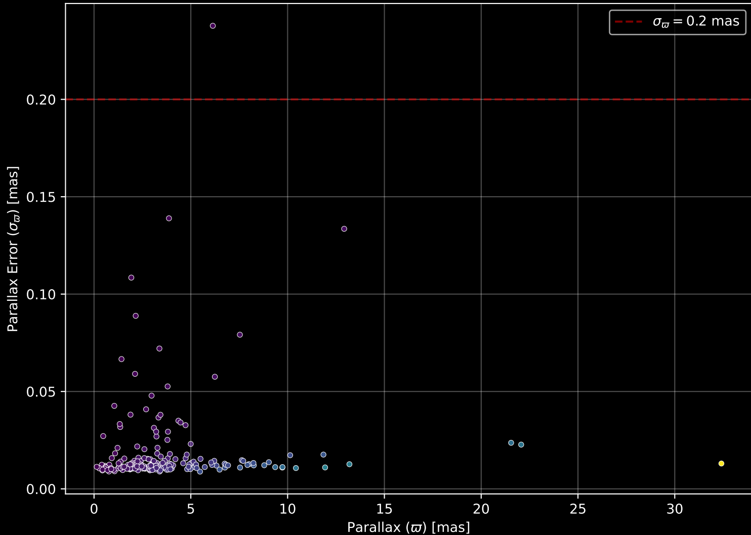
APOGEE DR17 Field: [082+57_MGA] Parallax Quality (n= 210)
