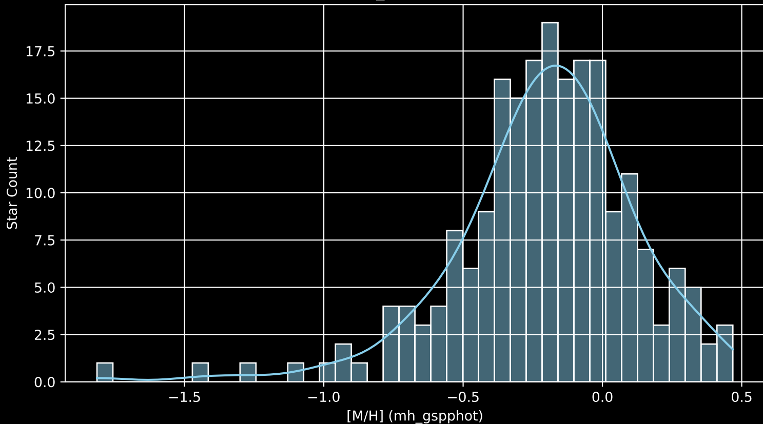
APOGEE DR17 Field: [082+57_MGA [M/H] (mh_gspphot) (n= 209)
